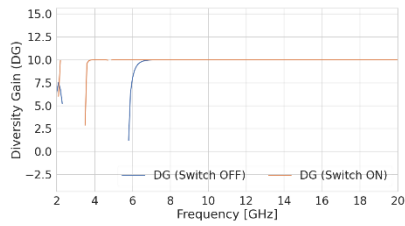
Fig 6. Diversity Gain (DG) in switched (a) ON and (b) OFF state (simulated) of the proposed eight-port SWB-MIMO antenna.
