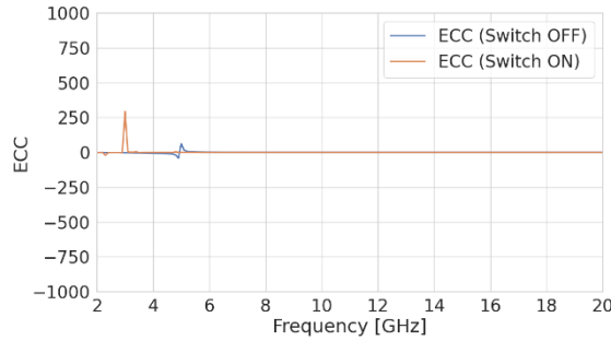
Fig 5. Envelope Correlation Coefficient (ECC) in switched (a) ON and (b) OFF state (simulated) of the proposed eight-port SWB-MIMO antenna.
