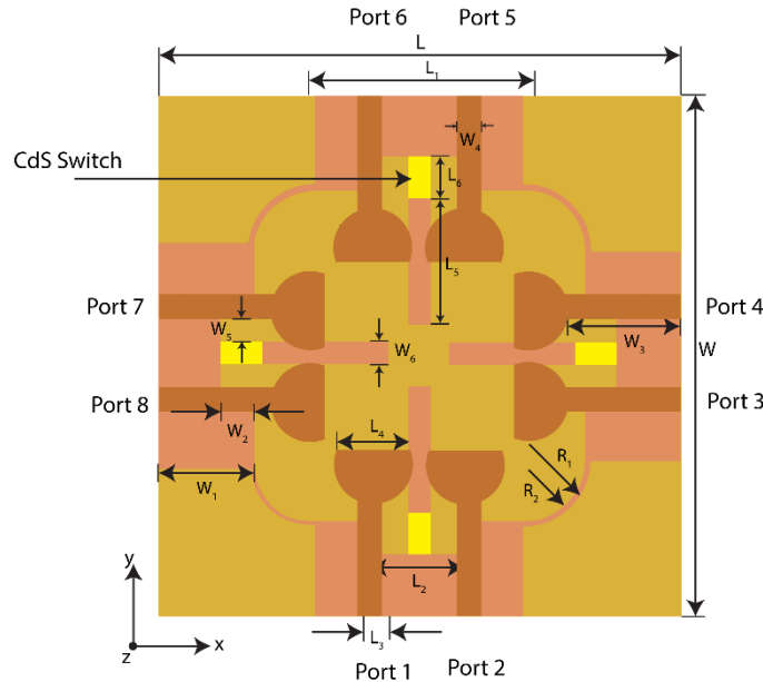
Fig 1. Geometry & design parameters of the proposed eight port SWB- MIMO antenna: [ L1=24mm , L2=10mm , L3=2.7mm , L4=10 mm , L5=13.75mm , L6=5mm , W1=10 mm , W2=5mm , W3=12.5mm , W4=0.4mm , W5=4mm , W6=2mm , R1=7.2mm , R2=6.5mm , R3=4.2mm ]
