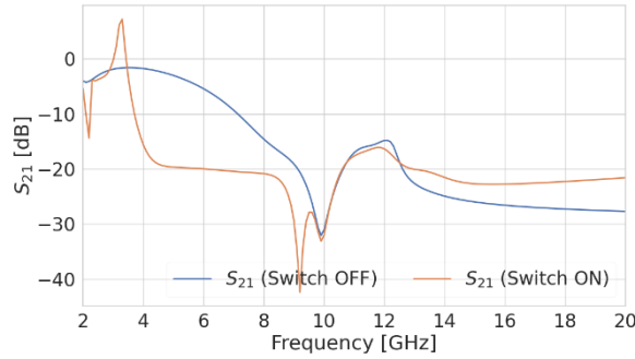
Fig 3. S_{21} Performance of the reconfigurable 8 port MIMO antenna.
